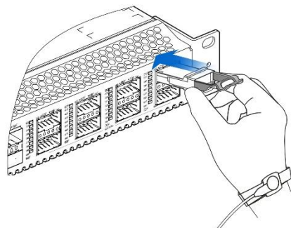
Figure 6-14 Installing the OSFP Transceiver with a Pull-Tab
