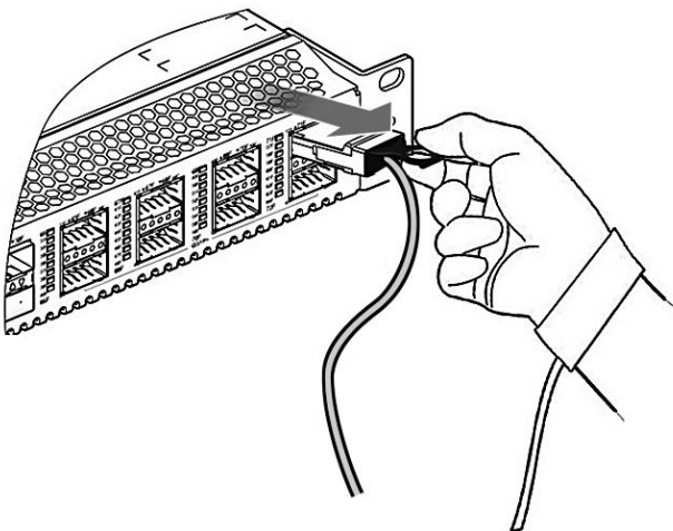
Figure 6-12 Removing the QSFP+ AOC Transceiver
