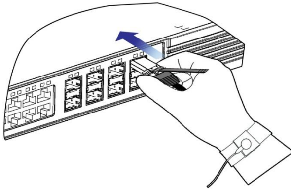
Figure 6-5 Installing the SFP28 AOC Transceiver
