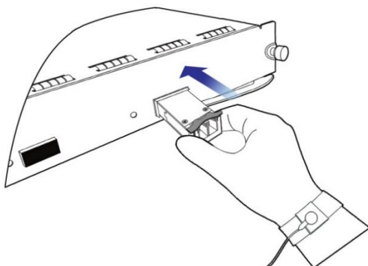
Figure 6-1 Installing the XFP Transceiver
